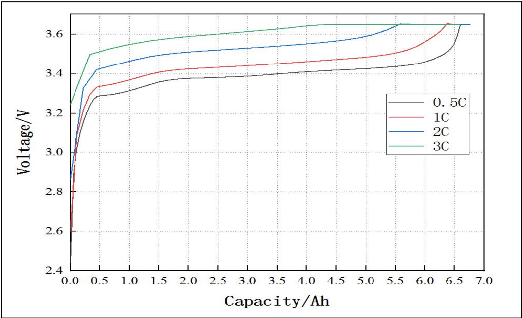
6.7Ah 磷酸铁锂系电池不同倍率充电曲线 Different rate charge curve of 6.7Ah LiFePO 4 cell
